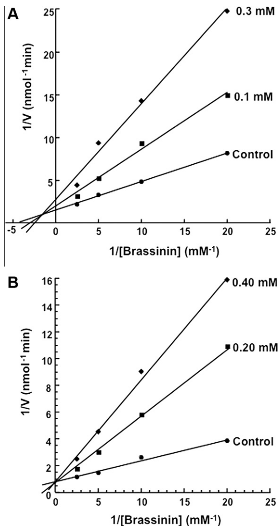
Figure 3. Lineweaver–Burk plots of BHAb activity. In the presence of (A) methyl naphthalen-1-yl-methylcarbonate ( 19 ) and (B) methyl naphthalen-2-yl-methylcarbonate ( 20 ).
