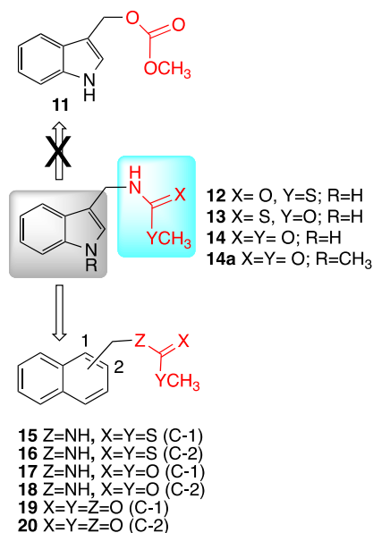
Scheme 2. Bioisosteres of brassinin (1) and corresponding naphthalenyl derivatives designed to probe the substrate specificity of BHAb.
