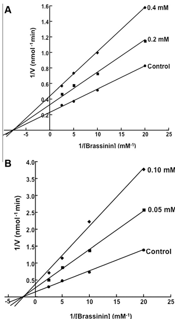
Figure 1. Lineweaver–Burk plots of BHAb activity. In the presence of (A) methyl N' -(1-methyl-3-indolylmethyl)carbamate ( 14a ) and (B) methylnaphthalen-1-yl-methylcarbamate ( 17 ).
