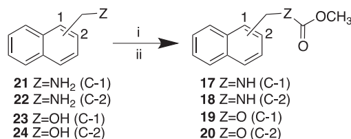
Scheme 3. Synthesis of 1- and 2-naphthalenylmethyl carbamates 17 and 18 and carbonates 19 and 20 . Reagents and conditions: (i) ClCO 2 Me, Et 3 N, CH 2 Cl 2 , rt, 17 (97%), 18 (96%); (ii) ClCO 2 Et, NaH, THF, 0 °C, 19 (80%), 20 (51%).
