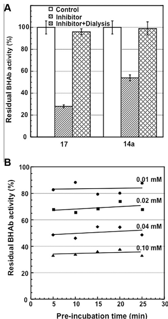
Figure 2. Characterization of the type of BHAb inhibition by methyl N' -(1-methyl-3-indolylmethyl)carbamate ( 14a ) (0.30 mM) and methyl naphthalen-1-yl-methylcarbamate ( 17 ). (A) Effects of methyl N' -(1-methyl-3-indolylmethyl)carbamate ( 14a ) (0.30 mM) or methyl naphthalen-1-yl-methylcarbamate ( 17 ) (0.1 mM) on BHAb activity after dialysis. (B) Time- and concentration-dependent activity of BHAb under increasing concentrations of methyl naphthalen-1-yl-methylcarbamate ( 17 ). Control experiments were performed in the absence of compounds (dialysis of the purified enzyme). Results are expressed as mean \pm standard deviation of three separate experiments.
