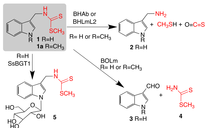
Scheme 1. Enzyme mediated transformations of brassinin ( 1 ): BOLm, brassinin oxidase from Leptosphaeria maculans (isolates virulent on canola) 7 ; BHLmL2, brassinin hydrolase from L. maculans (isolates virulent on brown mustard); BHAb, brassinin hydrolase from Alternaria brassicicola 1 ; SsBGT1, brassinin glucosyl transferase from Sclerotinia sclerotiorum . 8
